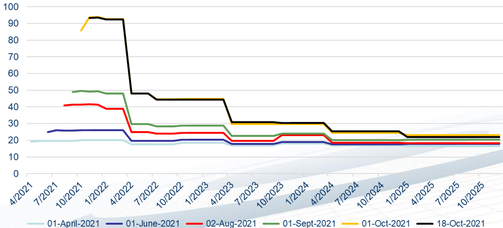
EEX CEGH Futures Price Curve on a given day (EUR/MWh)
